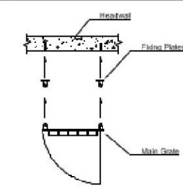
Frontwall Grate Fixing Detail Plan (NTS)
