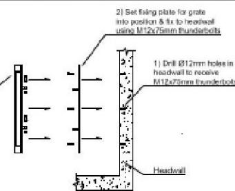
Frontwall Grate Fixing Detail Section (NTS)
