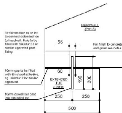
Extended Toe Fixing Detail (Scale 1:20)
