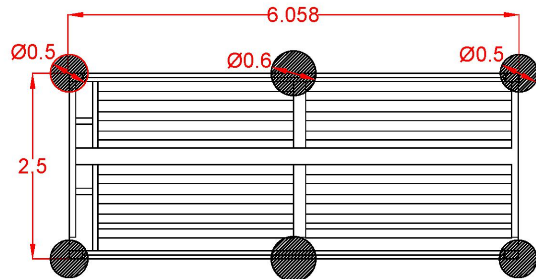
BOTTOM VIEW
