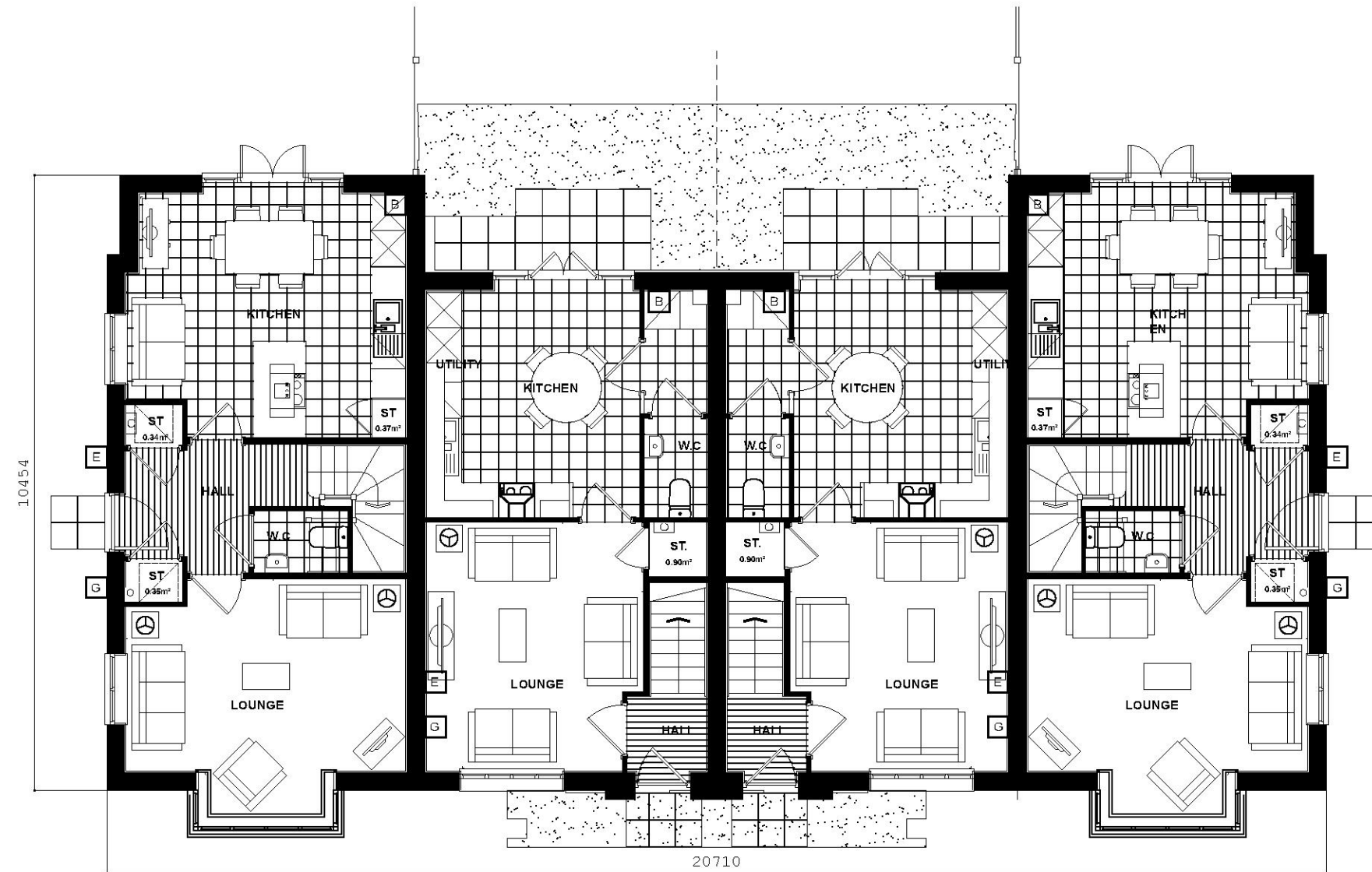
GROUND FLOOR PLAN MACAULAY
