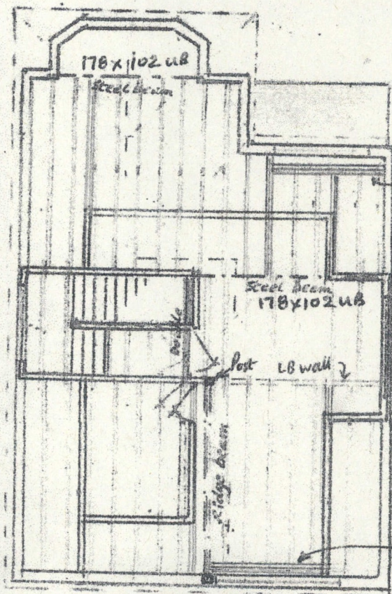
SECOND FLOOR PLAN. (Floor joist & beam layout)
