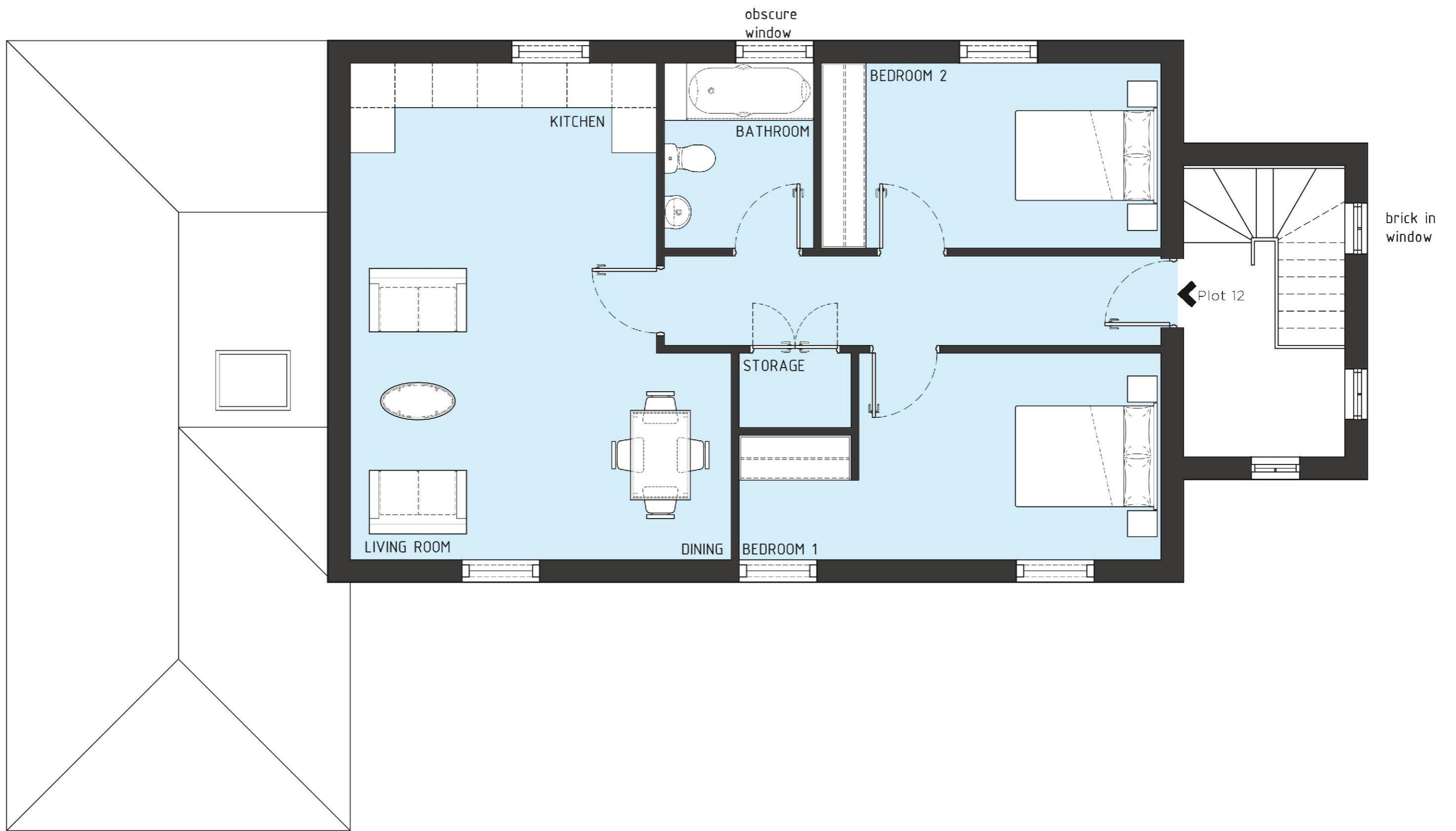
AS PROPOSED FIRST FLOOR PLAN
