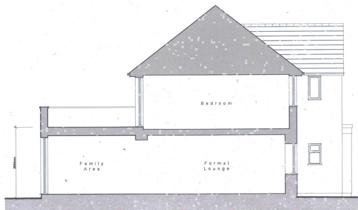
PROPOSED INDICATIVE SECTION 1:100
