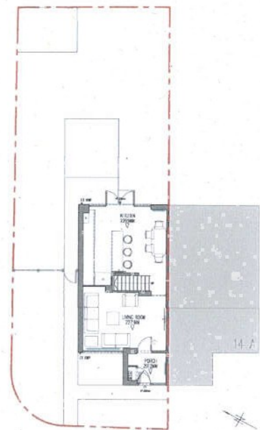
1 EXISTING GROUND FLOOR PLAN 1:100
