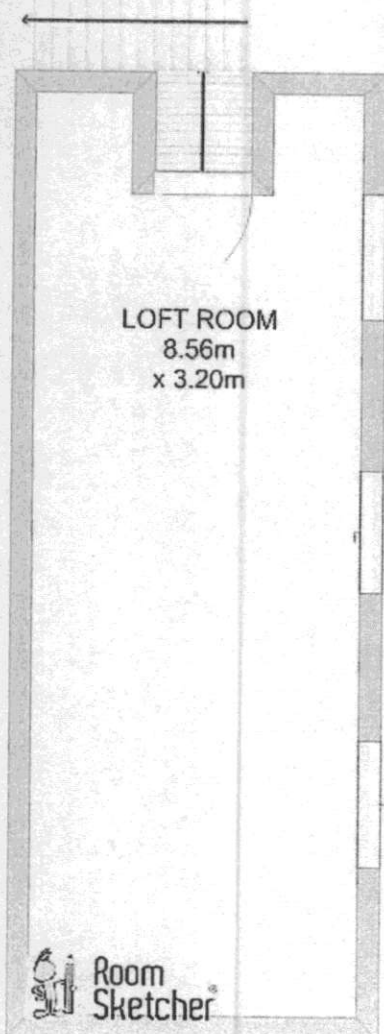
EXISTING LEVEL 2 FLOOR PLAN – TO BE UNCHANGED
