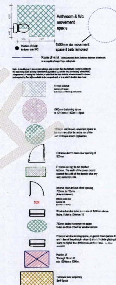
NOTE :- Symbols not to scale
