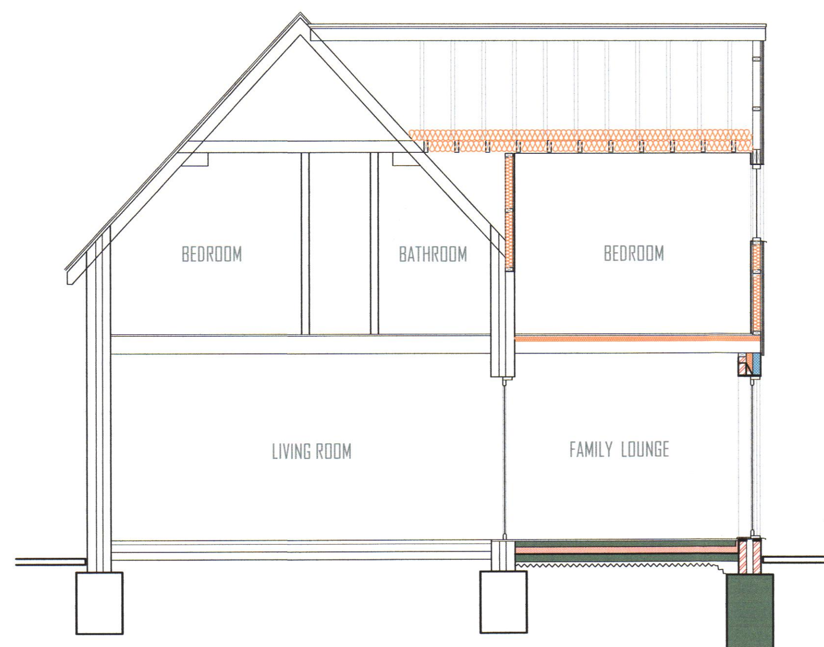
SECTION Scale 1:50
