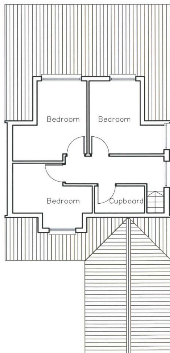
02 First Floor Plan SCALE 1/100
